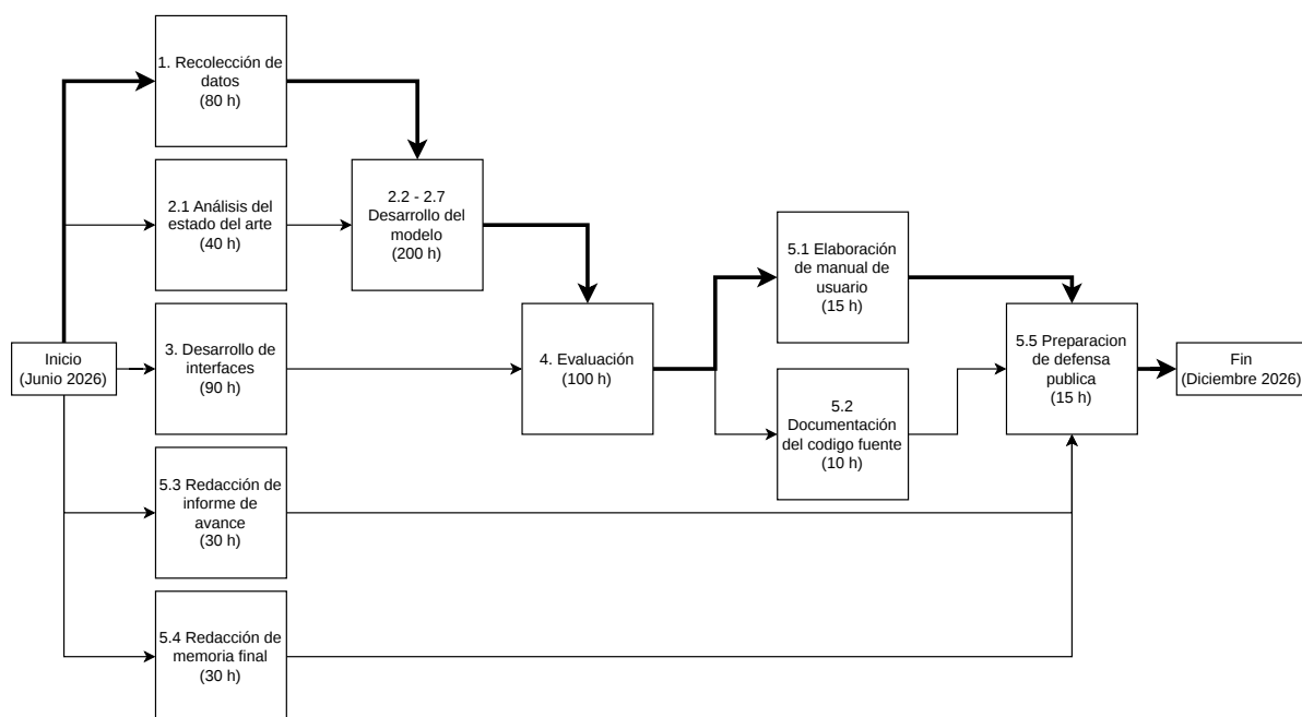
Figura 3. Diagrama de Activity on Node .
