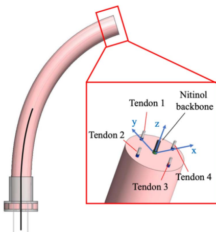
Figura 1. Robot Flexible
